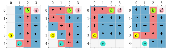
Fig. 3: A summary of the synthesized policy for the nursery scenario. Arrows: actions top , left , down , and right ; encircled characters: state labels. The actions in states that are not reachable or lead to another LDBA state are not displayed. In all subfigures, the most likely paths are highlighted in red.
